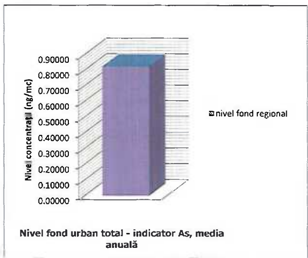
Figura nr. III-33Nivel Fond urban total – indicator As
