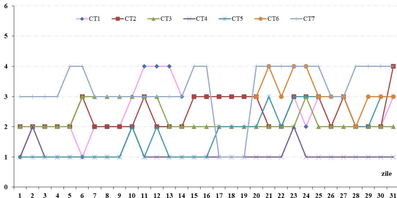
Indici generali - august 2020
