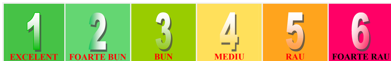
Indici generali - august 2020
