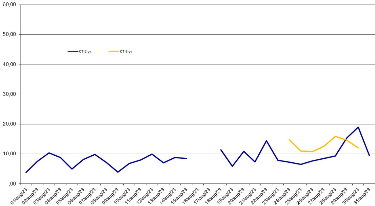
PM2.5 gv (ug/m3), perioada: 01 - 31 August 2023 - Date validate
