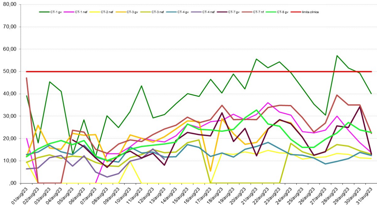
PM10 nef si PM10 gv (ug/m3), perioada: 01 - 31 August 2023 - Date validate
