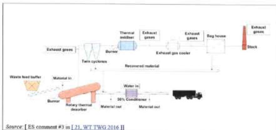
Figure 5.21: Example of a rotary thermal desorber installation
