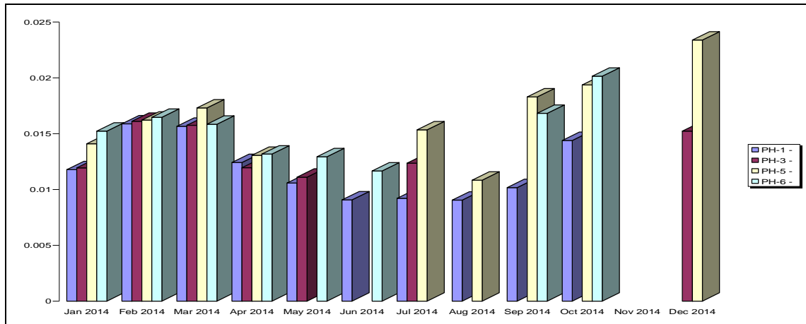
Channel: Pb10grv (ng/m3), period: 01 Jan 2014-31 Dec 2014 - Validate data
