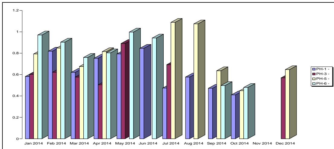
Channel: As10grv (ng/m3), period: 01 Jan 2014-31 Dec 2014 - Validate data
