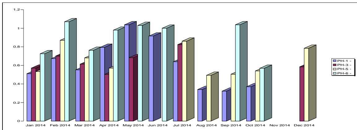
Channel: Cd10grv (ng/m3), period: 01 Jan 2014-31 Dec 2014 - Validate data
