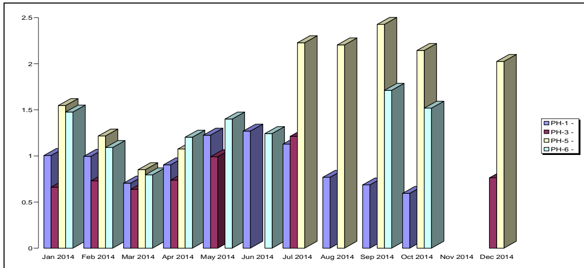
Channel: Ni10grv (ng/m3), period: 01 Jan 2014-31 Dec 2014 - Validate data
