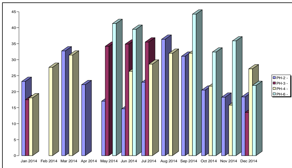
Channel: O3 (ug/m3), period: 01 Jan 2014-31 Dec 2014 - Validate data
