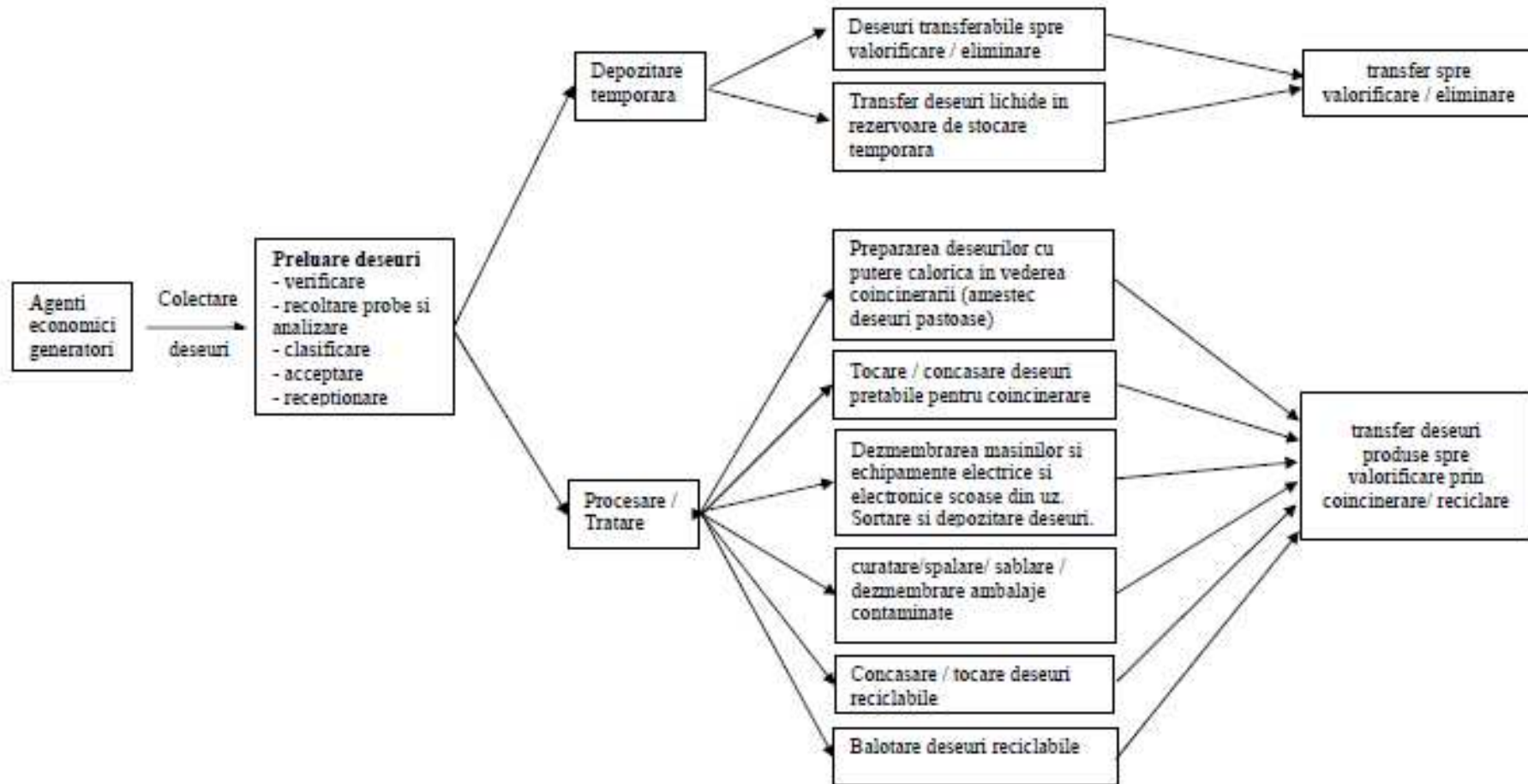
Figura 3: Schema flux tehnologic JIFA SRL
