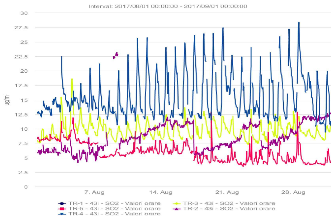
Fig. 1.1 - SO 2 ( \mu\text{g}/\text{m}^3 ), August 2017
