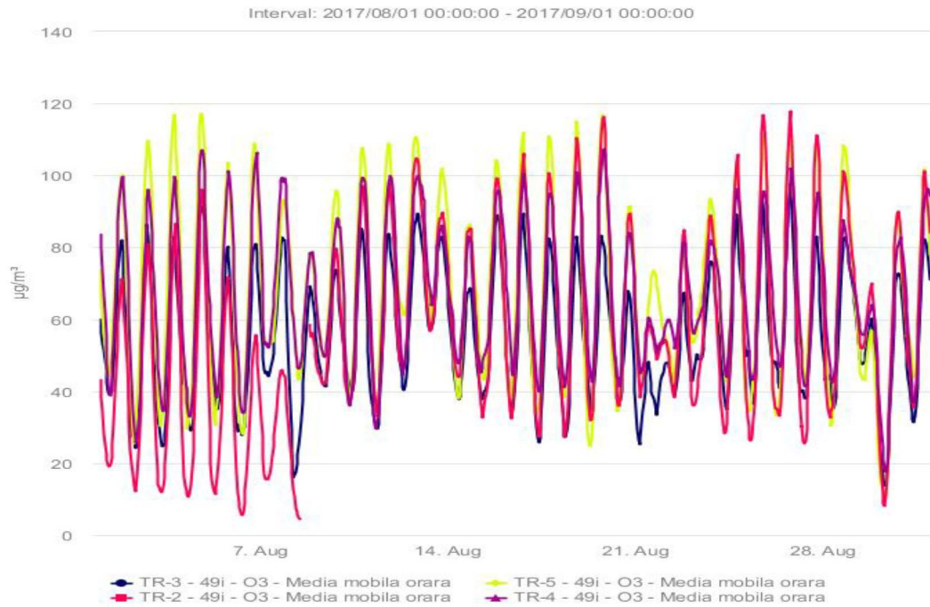
Fig. 1.3 - \text{O}_3 ( \mu\text{g}/\text{m}^3 ), August 2017
