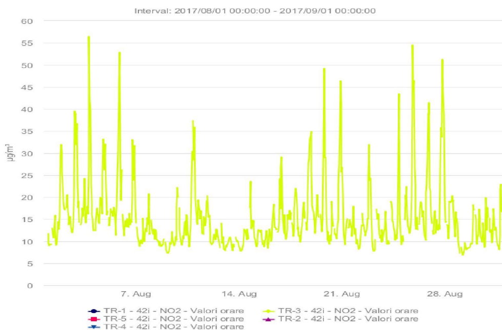
Fig. 1.2 - NO 2 ( \mu\text{g}/\text{m}^3 ), August 2017
