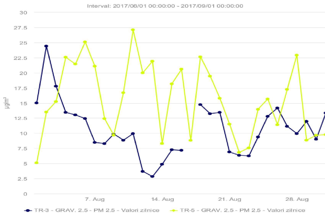
Fig. 1.6 – PM2.5 ( \mu\text{g}/\text{m}^3 ), August 2017
