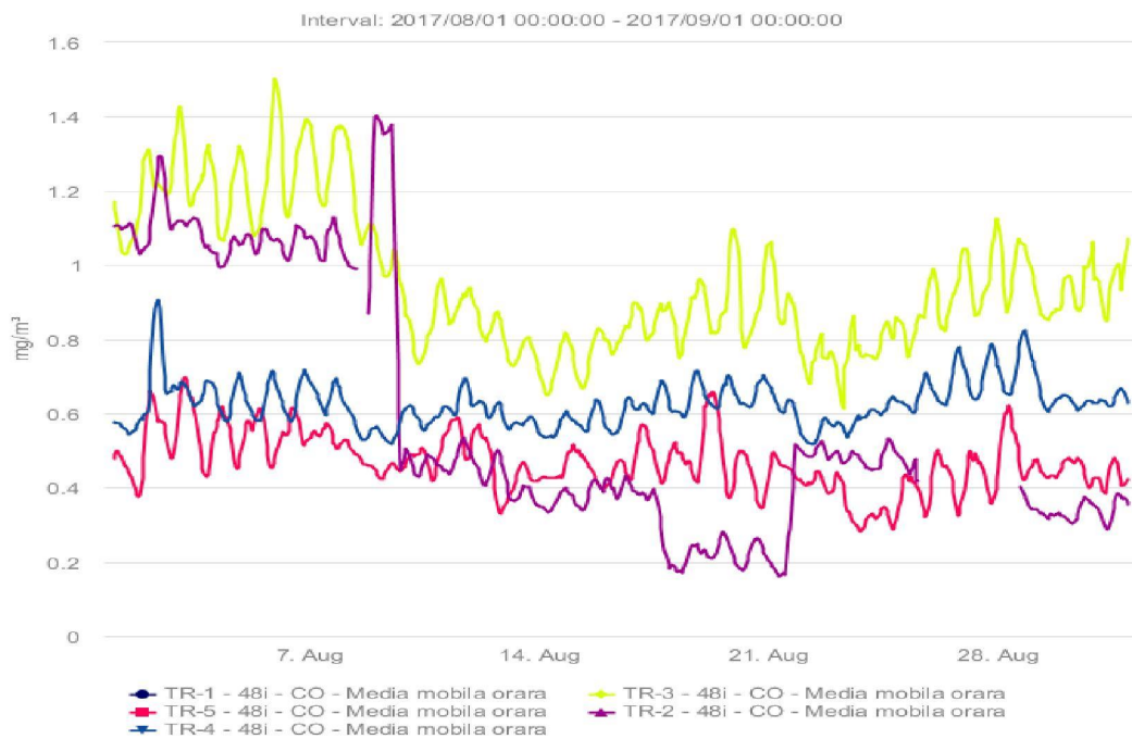
Fig. 1.4 - CO ( \text{mg}/\text{m}^3 ), August 2017
