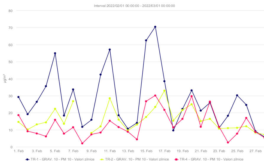
Fig. 1.7 – PM10 gravm. ( \mu\text{g}/\text{m}^3 ) – Februarie2022
