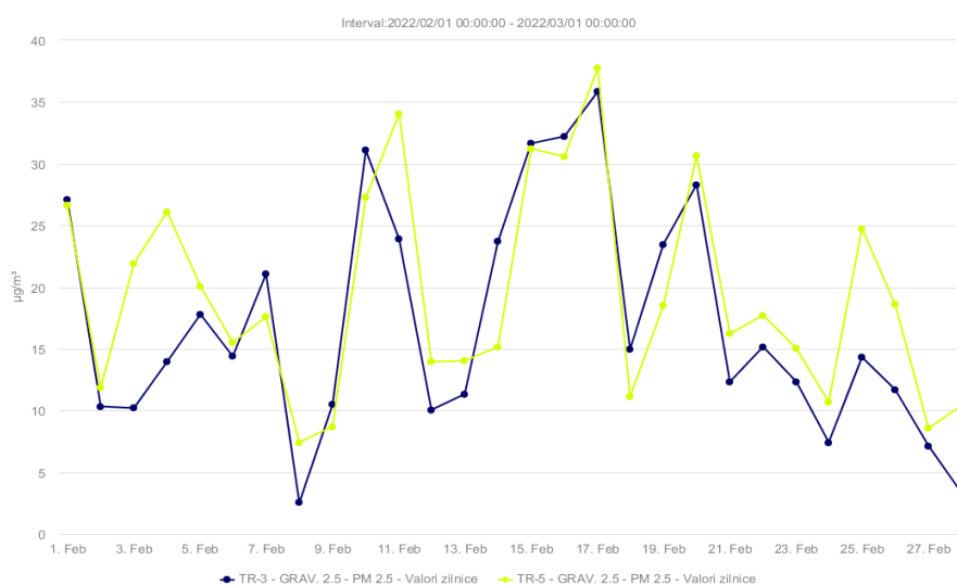
Fig. 1.8 – PM2.5 gravm. ( \mu\text{g}/\text{m}^3 ) – Februarie2022
