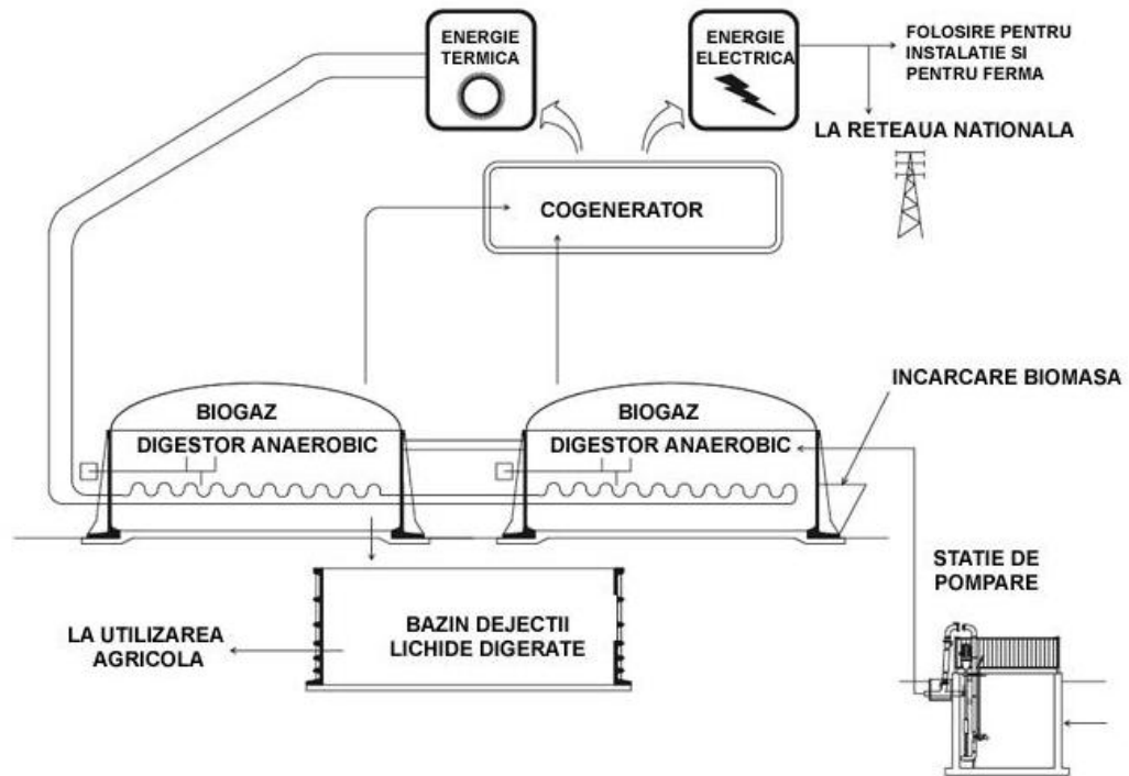
Fig.4- 6-SCHEMA INTRARI-IESIRI
