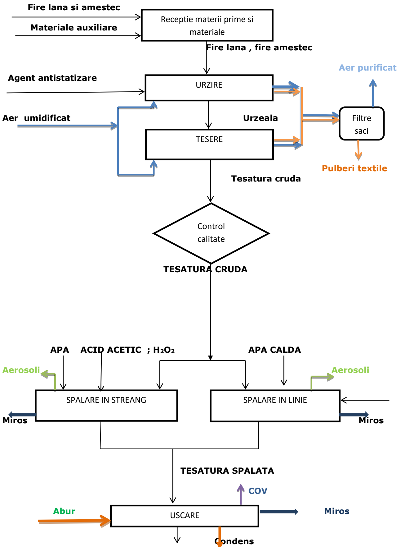
Diagrama flux producere tesaturi-Emisii in aer
