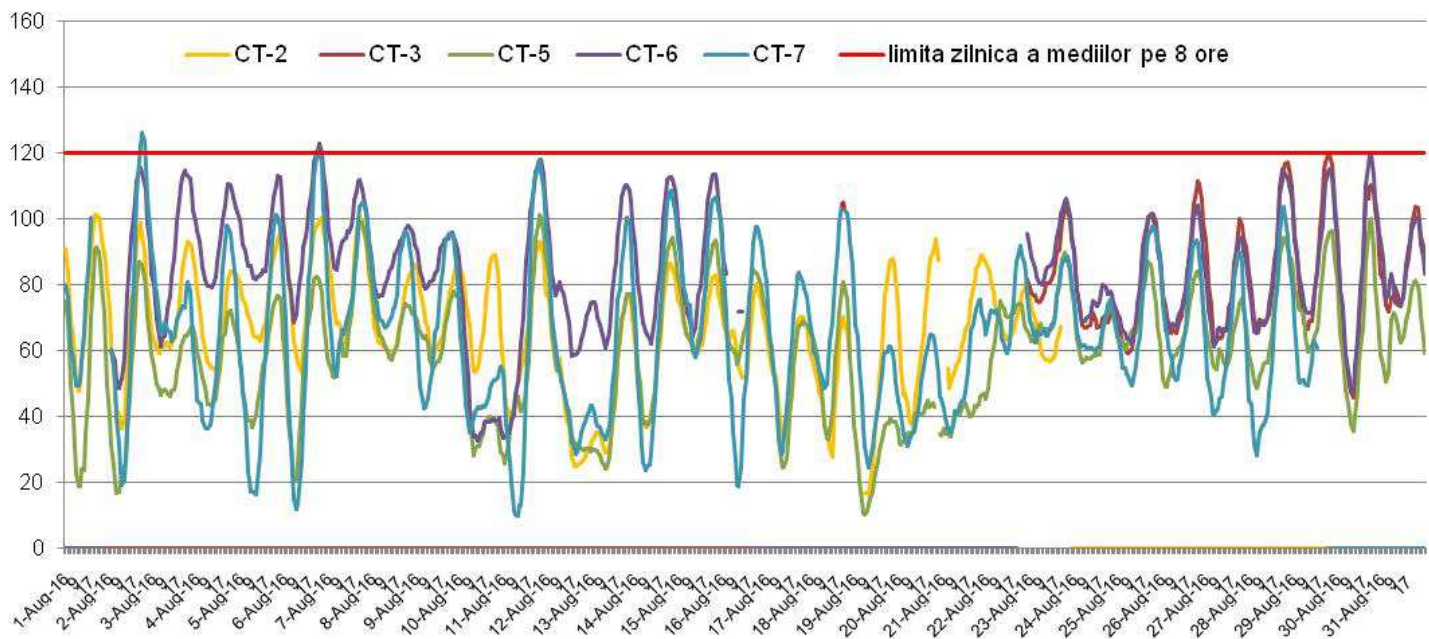
O 3 (ug/m 3 ), perioada: 01 Aug - 31 Aug 2016 - date validate
