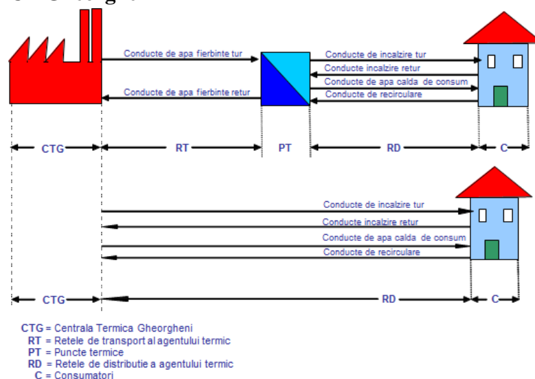
Fig. 5 Structura SACET – CT Gheorgheni
